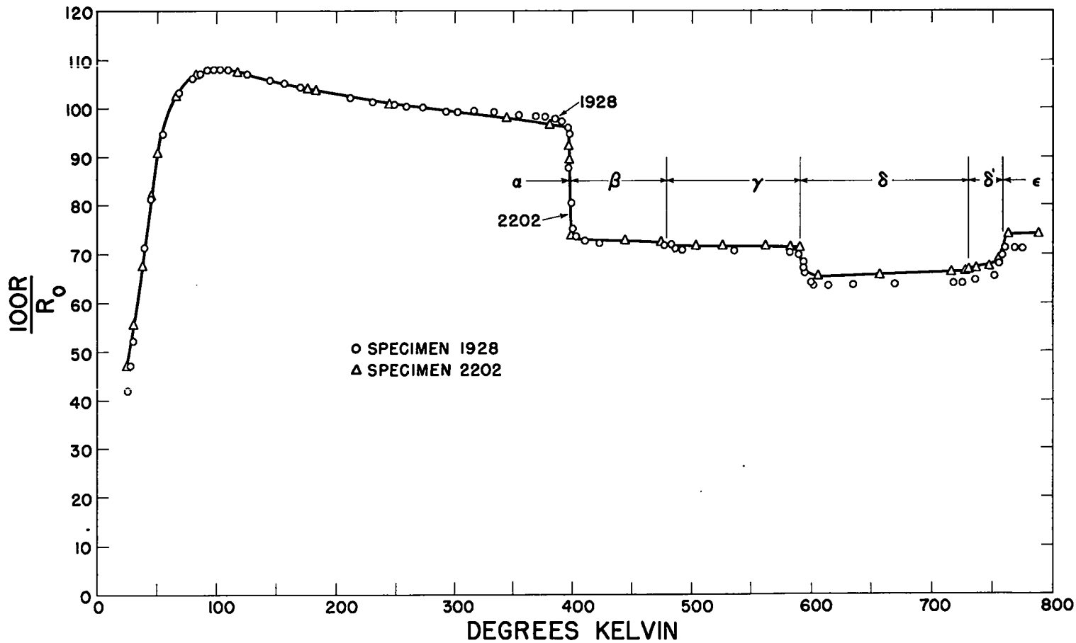
Fig. 2. 100R/R_0 vs absolute temperature for plutonium specimens.
