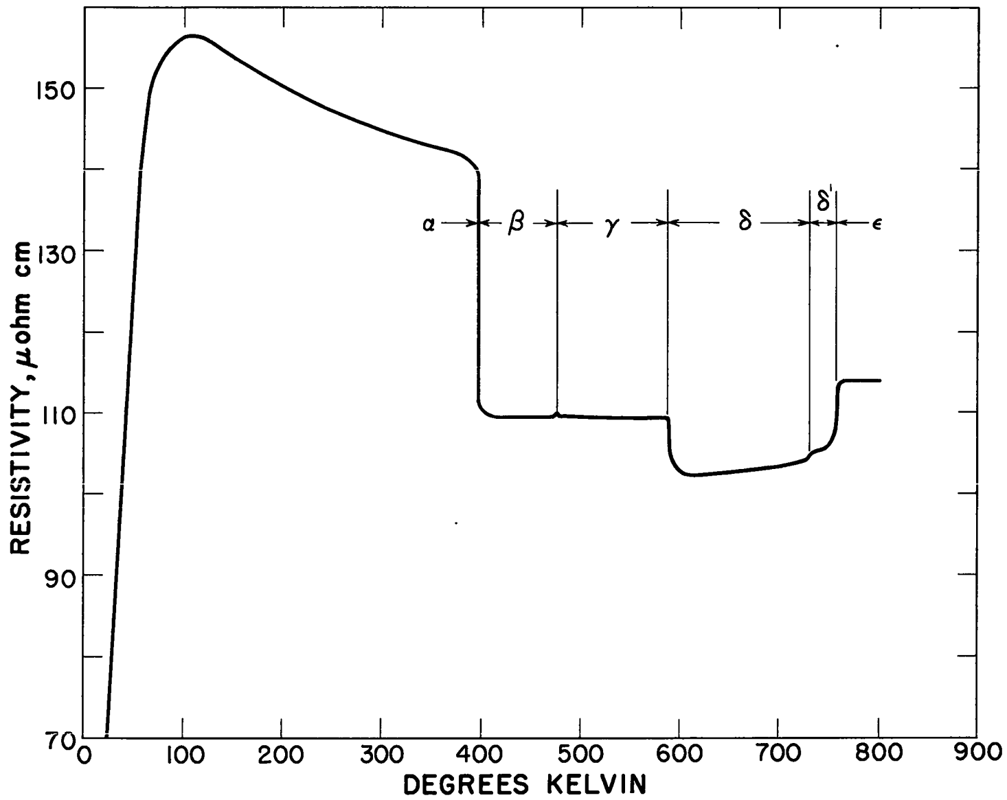
Fig. 3. Electrical resistivity of plutonium vs absolute temperature (specimen 2202).
