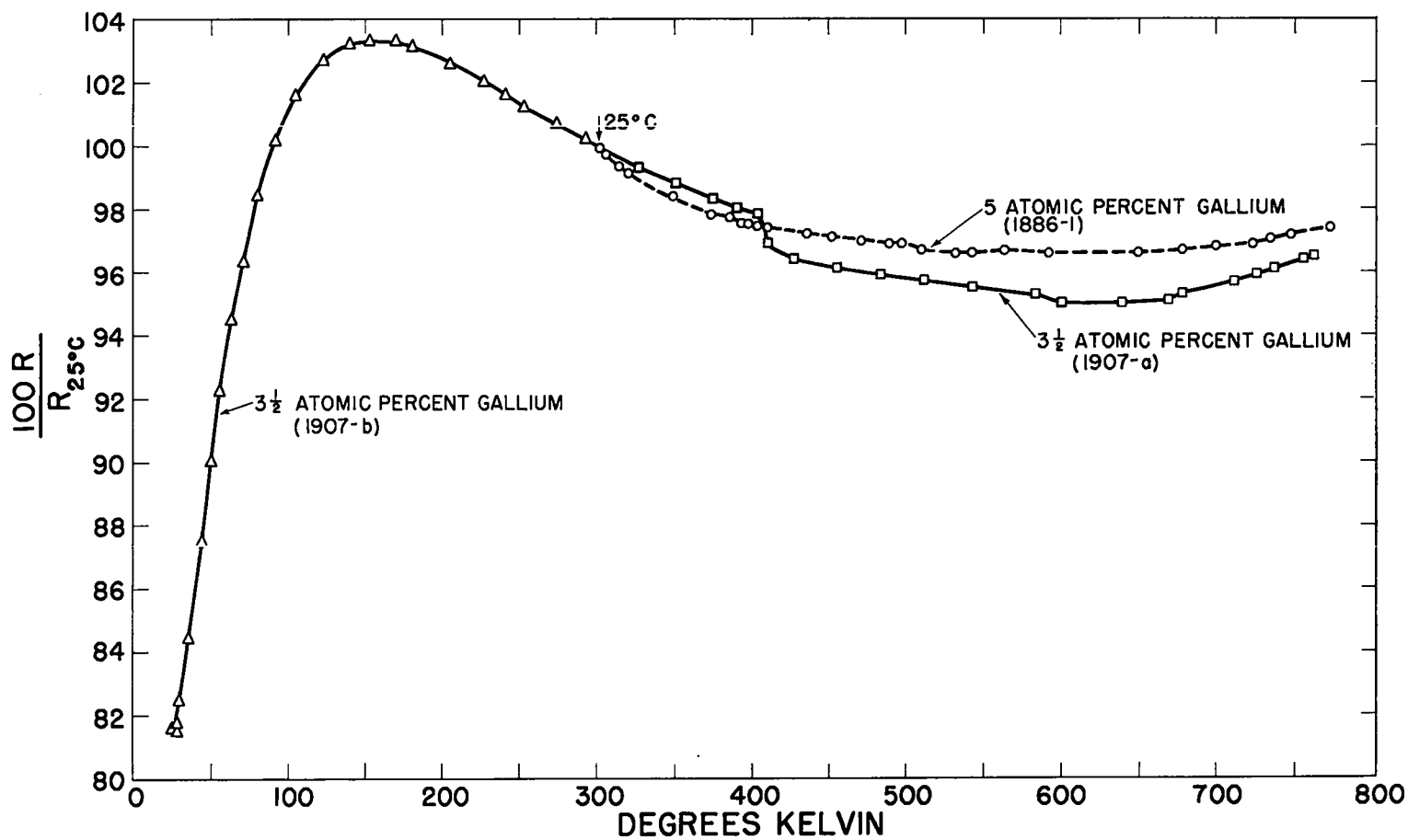
Fig. 4. 100R/R_{25^{\circ}C} vs absolute temperature for gallium-plutonium alloys.
