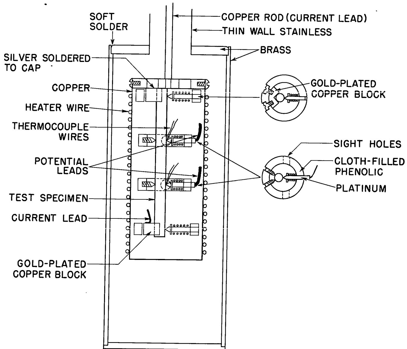
Fig. 1. Low-temperature electrical resistivity apparatus.
